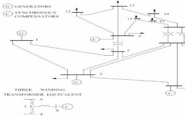
Figure 1: IEEE 14 Bus System
